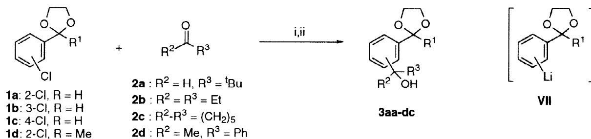
Scheme 1. Reagents and conditions: i, Li, C_{10}H_8 (10%), THF, -78^\circ C , 1 h; ii, H_2O , -78 to 20^\circ C .
